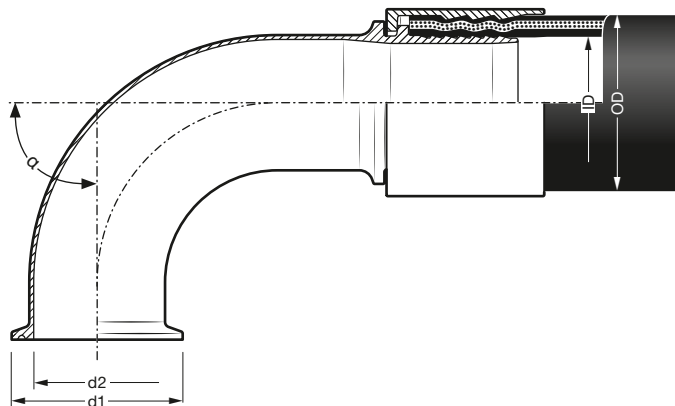
Type CFP ... -90°
